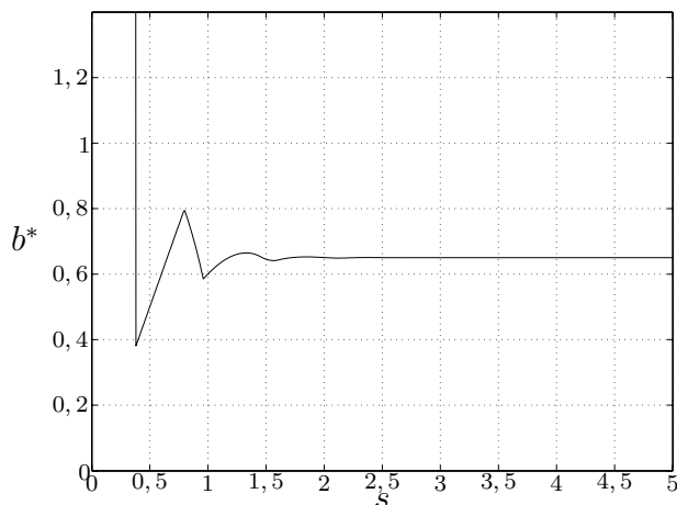
Figure 2: Optimal strategy for exponential distribution
