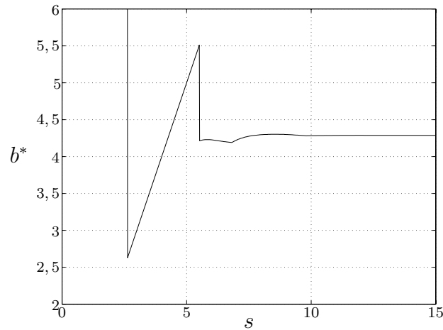
Figure 4: Optimal strategy for shifted exponential distribution
