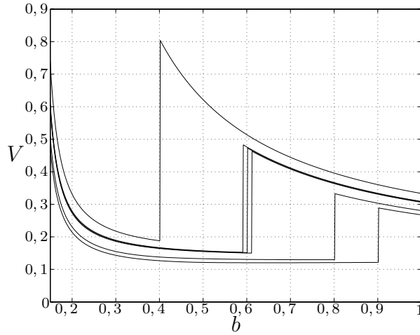
Figure 3: V(s, b) for different values of s and varying b
