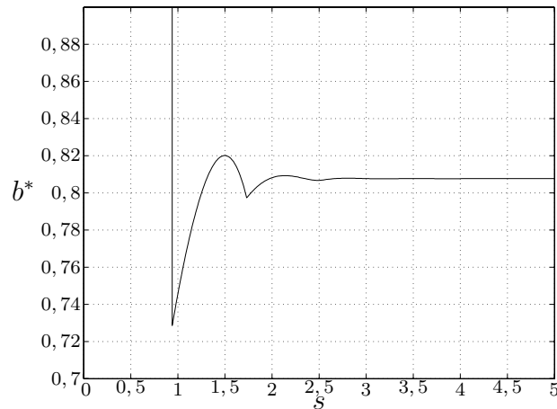
Figure 5: Optimal strategy for Pareto distribution
