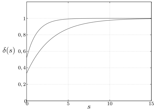
Figure 1: Survival probabilities
