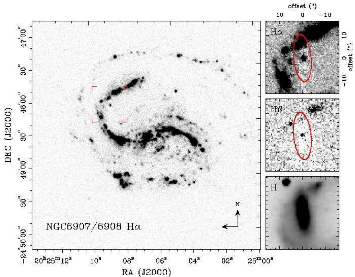
Fig. 3.— H \alpha image of NGC 6907/8. This continuum-subtracted image was obtained from the Anglo-Australian Telescope archive. The extent and the asymmetry of the spiral structure is especially noteworthy. At the position of NGC 6907 the image has been expanded (upper right panel) and two other wavelengths, continuum-subtracted H \beta (middle right panel) and the near-infrared H-band image (lower right panel) are shown for comparison. In the hydrogen-line images the overplotted ellipse shows the continuum outline of the main body of NGC 6908. Clearly the intruder shows nuclear emission in H \alpha and possibly in H \beta too.
