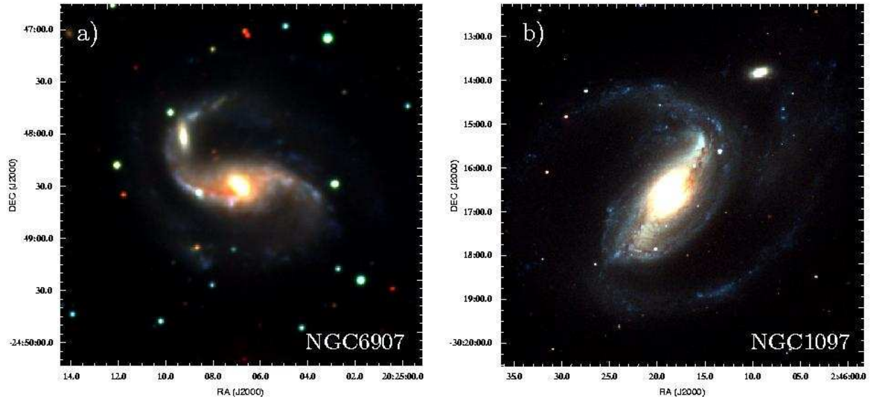
Fig. 5.— RGB color composite image of NGC 6907/08 produced by combining H (red), R (green), and B-band (blue) images. Note the difference in color between the North-West spiral arm of NGC 6907 and the S0 galaxy NGC 6908.
