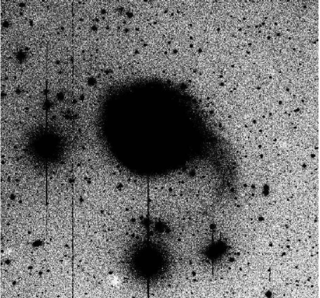
Fig. 7.— R-band CCD image of NGC 6907/8 taken with the duPont 2.5m at Las Campanas, Chile. The low-surface-brightness tidal feature to the south-west of the main galaxy is confirmed in this independent image, taken at a longer wavelength than the POSS (blue) image reproduced in Figure 6.
