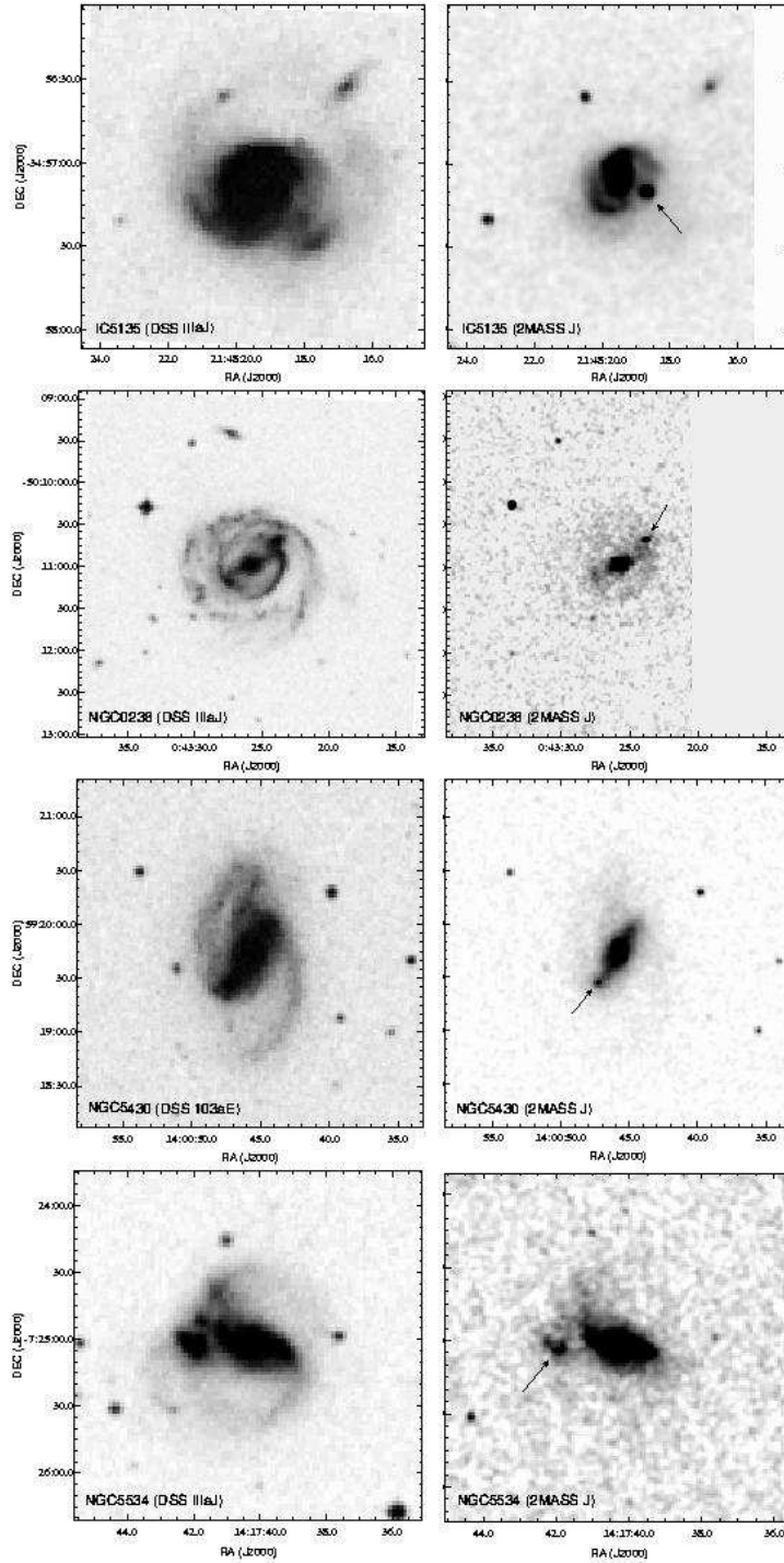
Fig. 8.— Selected examples of embedded companions discovered using long-wavelength archival images. The left-hand panels show optical images, right-hand panels show the near-infrared discovery images.
