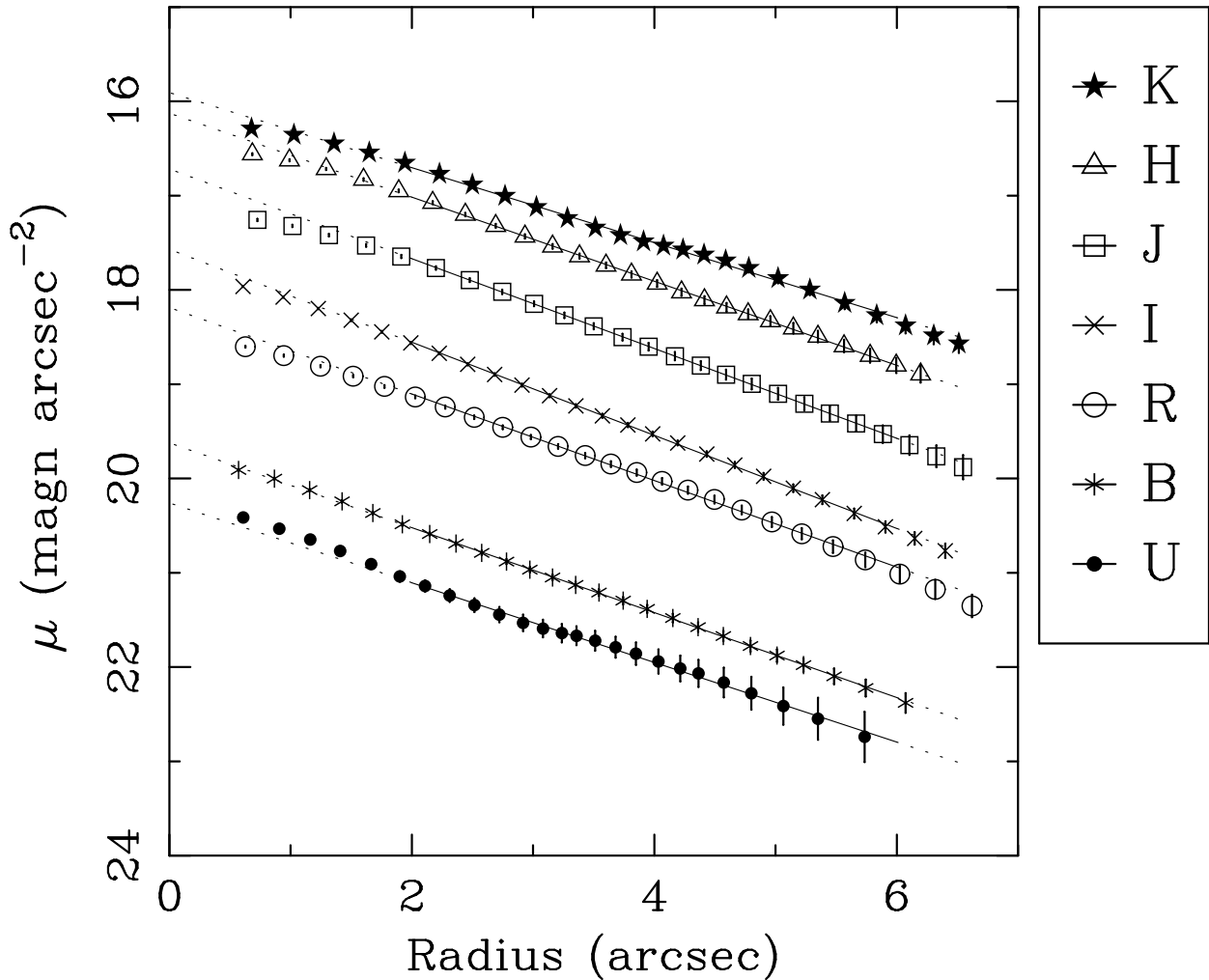
Fig. 2.— This figure shows the multi-wavelength radial light profiles of NGC 6908 derived from concentric elliptical isophote fitting. As can be readily seen, the fall-off is exponential from the near-ultraviolet (U-band: bottom profile) well out to 2.2 microns (K-band: top profile) confirming that this object is an S0 disk-like system, not an elliptical galaxy. Best-fitting straight lines are shown (lines are shown solid within the ranges used for the fit and dotted outside).
