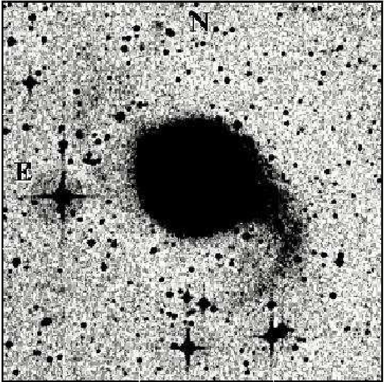
Fig. 6.— High-contrast POSS image of the outer regions surrounding NGC 6907/8. The one-armed spiral tail arcing from the north over to the west is clearly visible in this image. A more diffuse region of tidal debris is also visible to the north-east of the merging pair, arcing over to the northern edge of the image. The full field of view is 10 arcmin.
