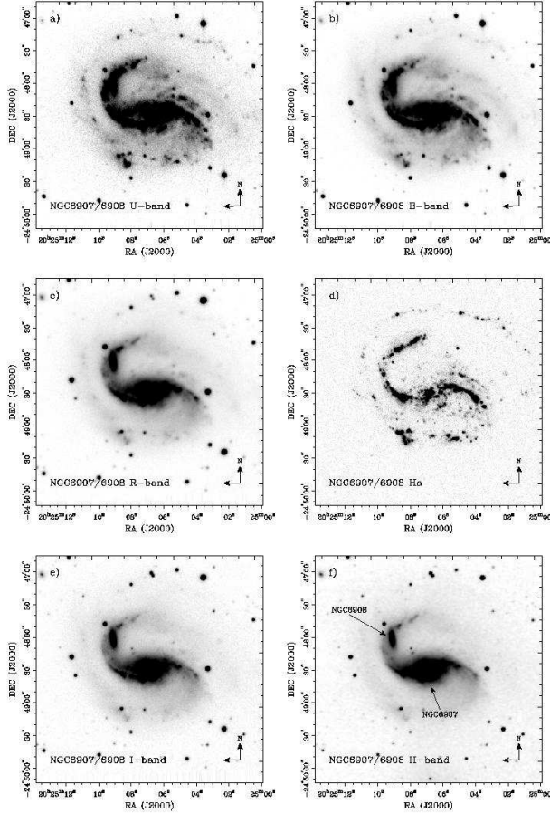
Fig. 1.— A multi-wavelength comparison of images of NGC 6907 and NGC 6908 from the blue to the near infrared. The upper two panels are U and B exposures respectively. In both cases one can see the “massive” eastern (left) arm emphasizing the asymmetry in the spiral structure of the dominant galaxy NGC 6907. In the middle left (R-band) image the composite nature of the eastern arm is beginning to become apparent as the elliptical form of NGC 6908 starts show itself. At progressively longer wavelengths (I and H-band images in the lower two panels) the contrast between the (red) companion and the (blue) spiral arm becomes even more enhanced and the companion is obvious beyond question. The middle right panel is a continuum-subtracted H\alpha image of the system. For all intents and purposes, the intruder, NGC 6908 has disappeared; but its effect are still rather dramatically present in the obvious discontinuity in the eastern arm delineated by the HII regions. At the position of NGC 6908 there is an abrupt change in the pitch angle of the arm and beyond that point the HII regions take up a distinctly linear formation behind the intruder. Finally, it is noteworthy to point out the finely delineated arc of HII regions that define the outermost parts of the spiral structure of NGC 6907. They complete a full 360deg wrapping of the optically less prominent western arm. In terms of bulk luminosity the eastern arm is dominant, but for total angular extent the western arm is by far the most extensive. For an expanded view of the H\alpha image see Figure 3. A RGB map of the BR and H-band images is shown in Figure 5.
