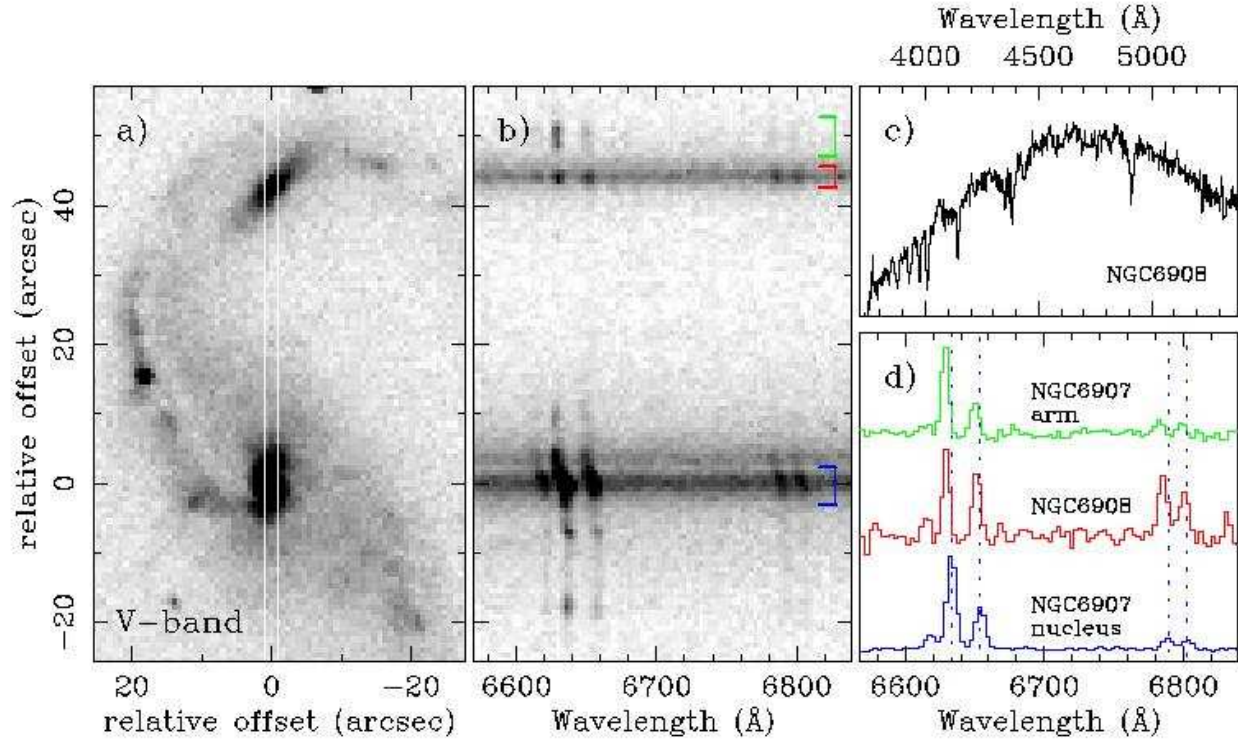
Fig. 4.— Long-Slit Spectra of NGC 6907 and NGC 6908. The left panel (a) shows the position of the 2-arcsec-wide slit used at the duPont 2.5m telescope superimposed on a V-band images of the two galaxies. The central panel (b) shows the sky-subtracted region of the spectrum (at the same spatial scale as panel a) used to determine the radial velocities, expanded to show only the wavelength region around H \alpha and the two sulfur lines. Square brackets to the right show the regions extracted for the radial velocity determinations, including a nearby HII region just above NGC 6908. The upper right panel (c) shows the (unflux-calibrated) hydrogen absorption-line spectrum of NGC 6908 taken at the Magellan telescope; while the lower right panel (d) shows the extracted emission-line spectra for the three objects (obtained at the duPont telescope) where the dashed vertical lines show the central wavelengths of H \alpha , [NII], and the two sulfur lines for the nucleus of NGC 6907 projected up and across the lines for the other two objects whose velocities are visibly lower. Each of the emission-line spectra are scaled to H \alpha so as to show the increased relative strength of the [NII] and [SII] lines in the nucleus of NGC 6908.
