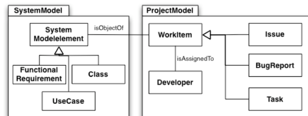
Figure 1: Excerpt from the unified model of UNICASE (UML class diagram)
