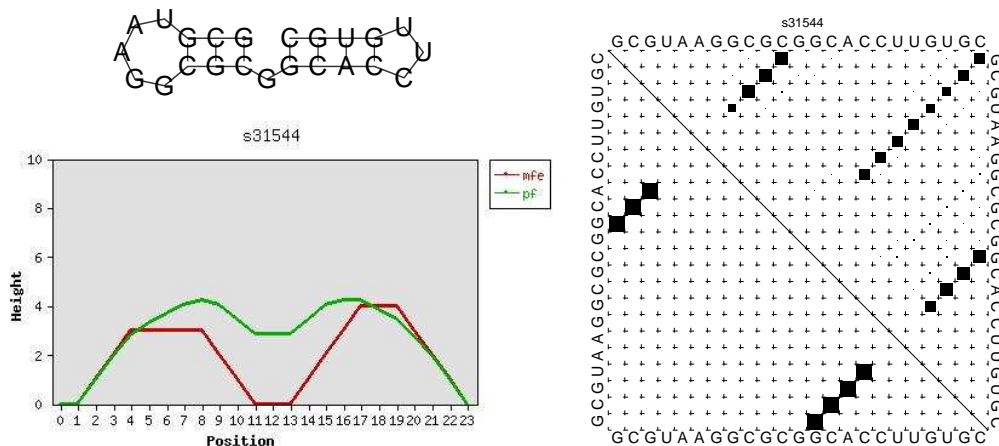
Figure 1. Three representations for secondary structure and structure ensembles as produced by the RNAfold service: Structure graph, mountain plot and dot plot. As can be seen clearly in the dot plot, the sequence has two almost equally good but very dissimilar foldings.
