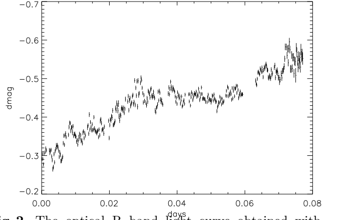
Fig. 2. The optical R band light curve obtained with a 1.2m telescope of Kryoneri station of the National Observatory of Athens covering 89% of the orbital period.
