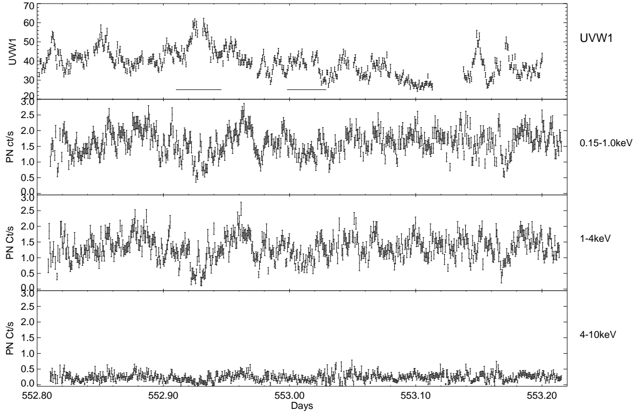
Fig. 1. The light curves of YZ Cnc, from the top; the UV data; 0.15–1.0 keV, 1–4 keV and 4–10 keV. The date is HJD-2452000.0. The bin size is 60 s. The times of anti-correlation between the X-ray and UV bands are shown with horizontal lines in the top panel.
