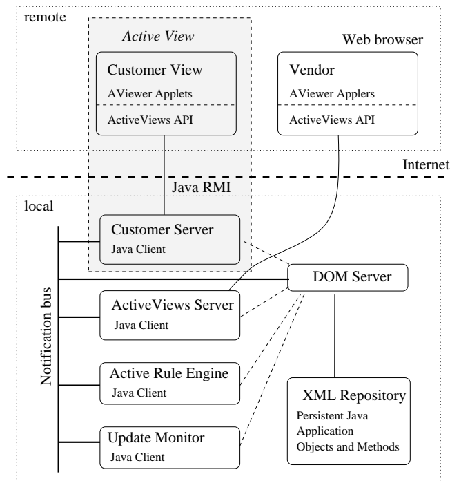
Figure 1: Demonstration Architecture
