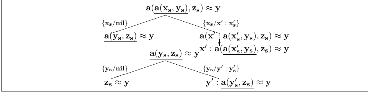
Figure 2: Normalizing lazy narrowing trees for \mathbf{a}(\mathbf{a}(\mathbf{x}_s, \mathbf{y}_s), \mathbf{z}_s) \approx \mathbf{y} and \mathbf{a}(\mathbf{x}_s, \mathbf{y}_s) \approx \mathbf{y} .
