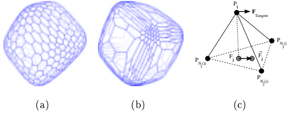
Fig. 9. (a) Deformable simplex mesh with reference metric parameters equal to 1/3 ; (b) Deformable simplex mesh with adaptation of its reference metric parameter in order to increase the resolution in places with high curvature; (c) Definition of the tangential force as (\tilde{F}_i - F_i) .
