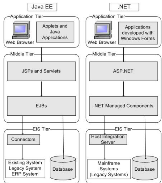
Fig. 3 Java EE and .NET tiers
