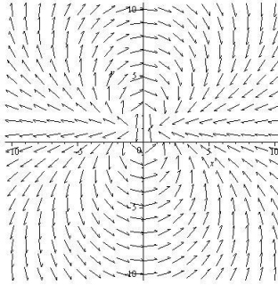
Fig. 1. The normal vector field of the rational system
