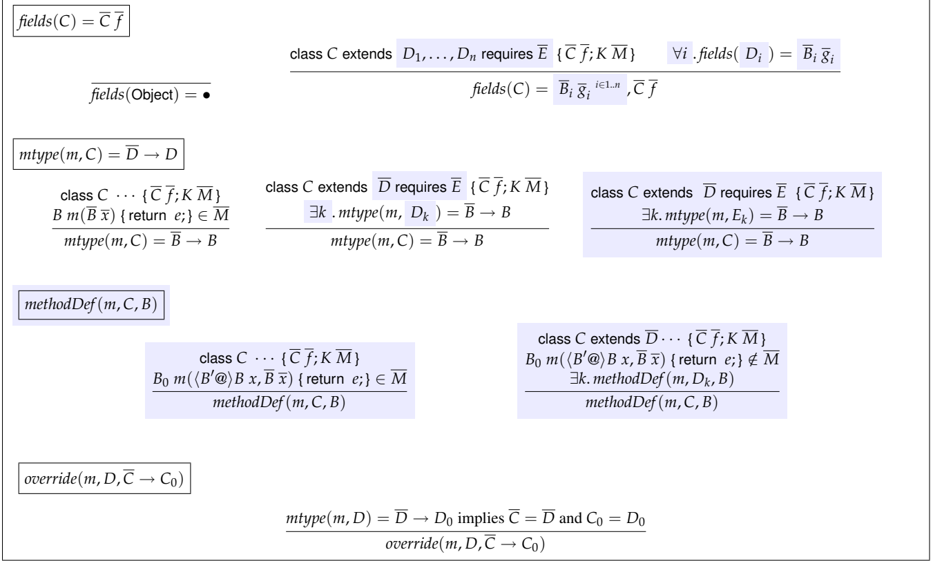
Figure 12. CZ typechecking auxiliary judgements
