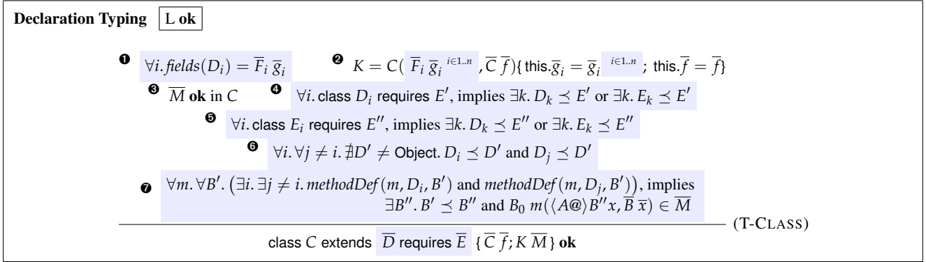
Figure 11. Class typing
