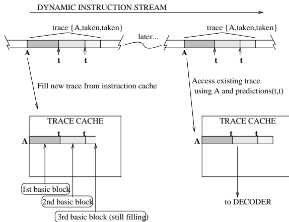
Figure 2. High level view of the trace cache.
