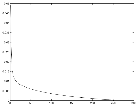
Figure 7: Plot of all 252 eigenvalues after applying globally normalized first derivative
