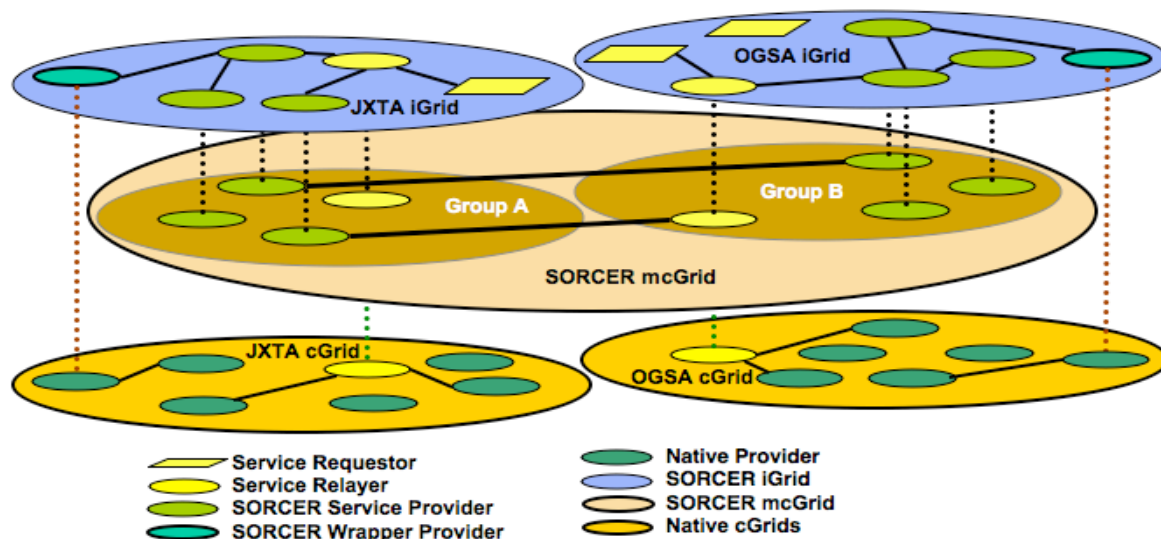
Figure 5: Integrating and wrapping cGrids with SORCER mcGrids. Two requestors, one in JXTA iGrid, one in OGSA iGrid submits exertion to a corresponding relayer. Two federations are formed that include providers from all the two horizontal layers below the iGrid layer (as indicated by continues and dashed links).
