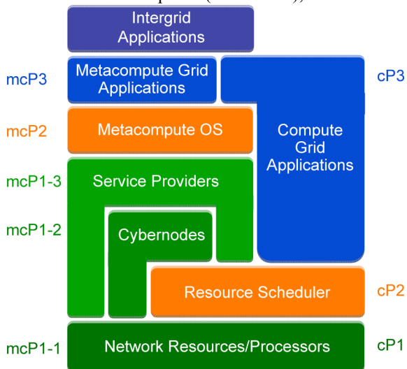
Figure 1: Three types of grids: compute grid, metacompute grid, and intergrid. A cybernode provides a lightweight dynamic virtual processor, turning heterogeneous compute resources into homogeneous services available to the metacomputing OS (“Project Rio”, n.d).
