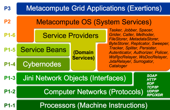
Figure: 3 SORCER layered platform, where P1 resources, P2 resource management, P3 programming environment
