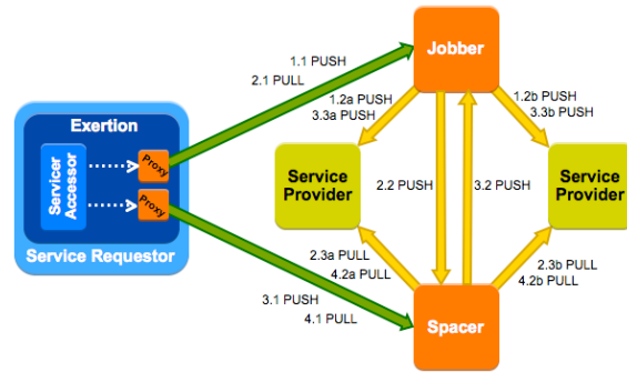
Figure 4: Push vs. pull exertion processing
