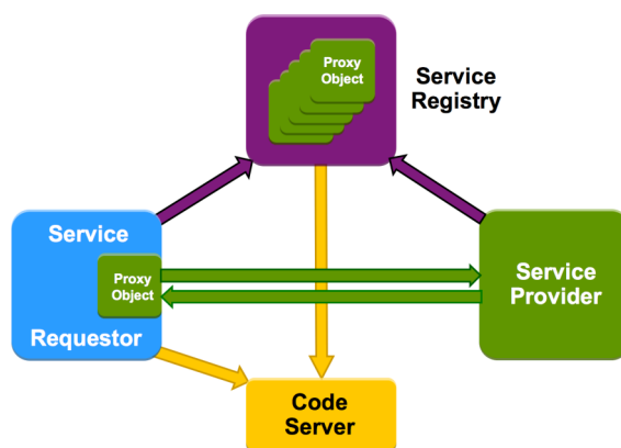
Figure 2: Service object-oriented architecture
