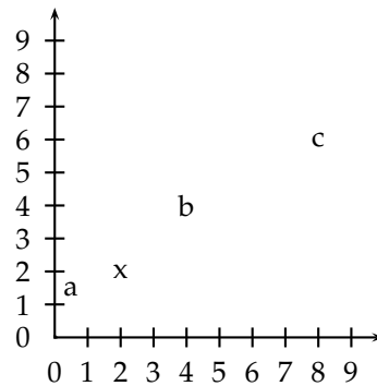
► Figure 14.12 Example for differences between Euclidean distance, inner product similarity and cosine similarity. The vectors are \vec{a} = (0.5 \ 1.5)^T , \vec{x} = (2 \ 2)^T , \vec{b} = (4 \ 4)^T , and \vec{c} = (8 \ 6)^T .
