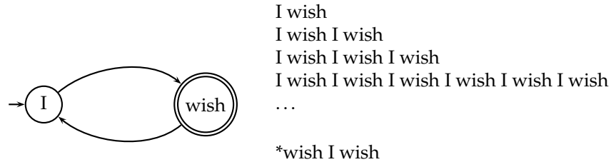
► Figure 12.1 A simple finite automaton and some of the strings in the language that it generates. → shows the start state of the automaton and a double circle indicates a (possible) finishing state.
