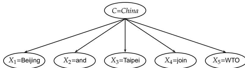
► Figure 13.5 The multinomial Naive Bayes model.
