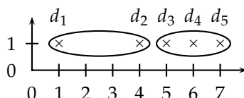
► Figure 17.7 Outliers in complete-link clustering. The five documents have the coordinates 1 + 2\epsilon , 4 , 5 + 2\epsilon , 6 and 7 - \epsilon . Complete-link clustering creates the two clusters shown as ellipses. The most intuitive two-cluster clustering is \{\{d_1\}, \{d_2, d_3, d_4, d_5\}\} , but in complete-link clustering, the outlier d_1 splits \{d_2, d_3, d_4, d_5\} as shown.
