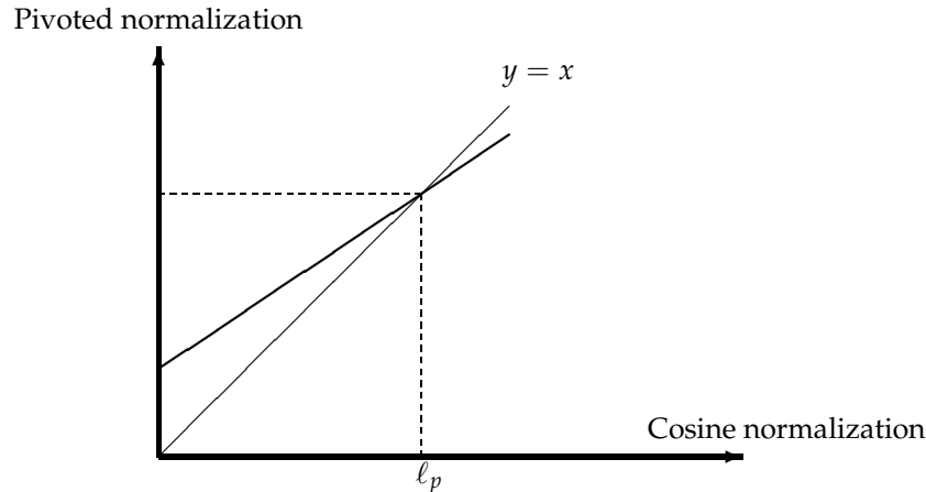
► Figure 7.5 Implementing pivoted document length normalization by linear scaling.
