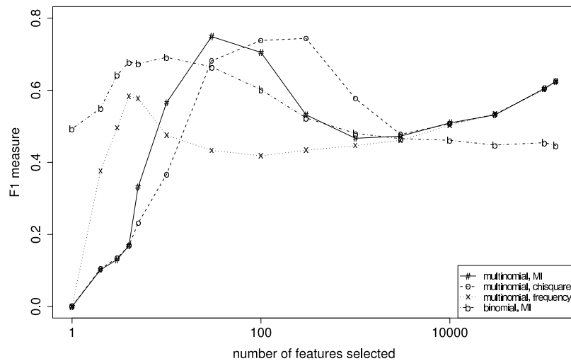
► Figure 13.9 Effect of feature set size on accuracy for multinomial and Bernoulli models.
