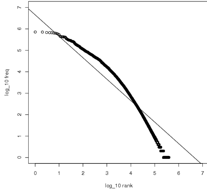
► Figure 5.9 Zipf's law for Reuters-RCV1. Frequency is plotted as a function of frequency rank for the terms in the collection. The line is the distribution predicted by Zipf's law.
