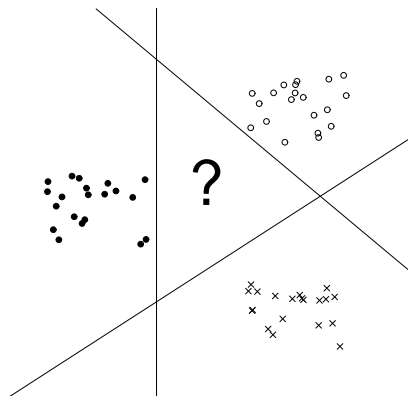
► Figure 14.11 J hyperplanes do not divide space into J disjoint regions.
