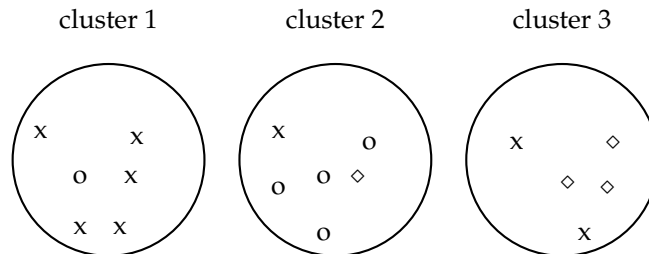
► Figure 16.4 Purity as an external evaluation criterion for cluster quality. Majority class and number of members of the majority class for the three clusters are: X, 5 (cluster 1); circle, 4 (cluster 2); and diamond, 3 (cluster 3). Purity is (1/17) * (5 + 4 + 3) \approx 0.71 .
