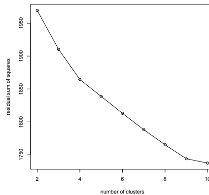
► Figure 16.8 Estimated minimal residual sum of squares ( \widehat{\text{RSS}} ) as a function of the number of clusters in k-means. In this clustering of 1203 Reuters-RCV1 documents, there are two points where the \widehat{\text{RSS}} curve flattens: at 4 clusters and at 9 clusters. The documents were selected from the categories China , Germany , Russia and Sports , so the K = 4 clustering is closest to the Reuters categorization.
