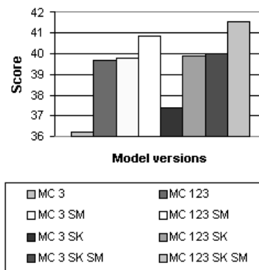
Figure 5: Exponential decay score for different Markov chain versions on transactions data set.
