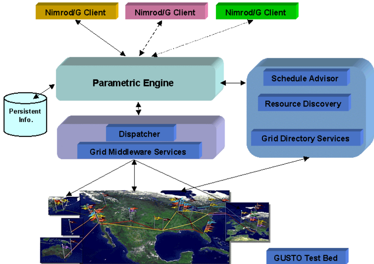
Figure 1. The Architecture of Nimrod/G
