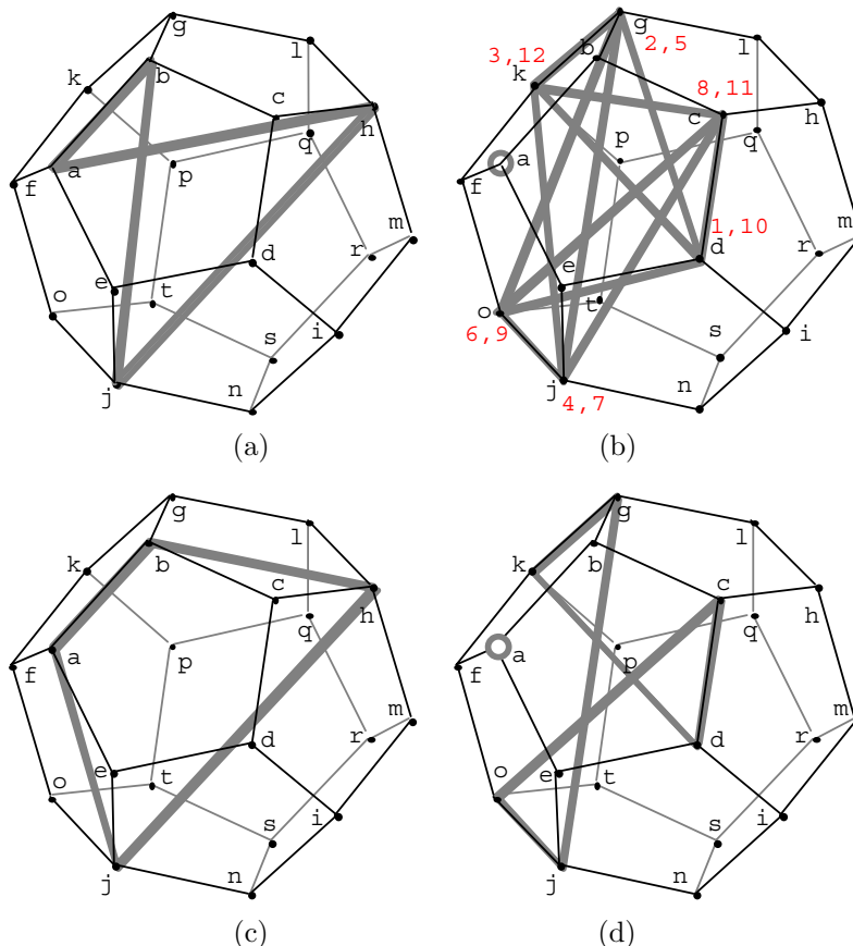
Fig. 12. Four noble polyhedra. The hexecontahedron in (a) consists of the sixty quadrangles congruent to the one emphasized, that can be inscribed in the regular dodecahedron. Its polar is an icosahedron, with twenty 12-gonal faces. The diagram in (b) shows the face which is the polar of the vertex a. Each of the 20 vertices of the icosahedron in (b) represents three coinciding vertices, while each face meets six pairs of coinciding vertices. Clearly, the coincidences here are no more against the traditional grain than the ones in the polyhedron in Figure 9. The other hexecontahedron is obtained similarly from the quadrangle in (c), while (d) shows the face of a noble icosahedron polar to the polyhedron in (c). The diagram in (d) shows the face which is the polar of the vertex a. Each of the 20 vertices of the icosahedron in (d) represents three coinciding vertices, while each face meets six pairs of coinciding vertices, each pair determining an edge of zero length. In all diagrams the dodecahedra serve only to guide the construction and recognition of the faces of the polyhedra described.
