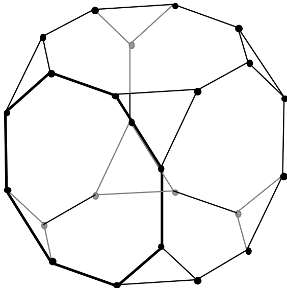
Fig. 14. Deleting all triangles from the uniform truncated cube (3 . 8 . 8), and then face-doubling the octagons, leads to two “new” polyhedra (8 . 8 . 8 . 8), which are not only uniform, but noble; moreover, they are isomegnetic. In both, each octagon has been replaced by one “red” and one “green” octagon. The two are adjacent along the four edges previously adjacent to triangles. In the first polyhedron the remaining edges are adjacent to octagons of the same color, in the second to differently colored ones. The difference between the two is that in the first, each triangular hole is surrounded by two circuits of three octagons each, while in the second one it is surrounded by one circuit of six octagons.
