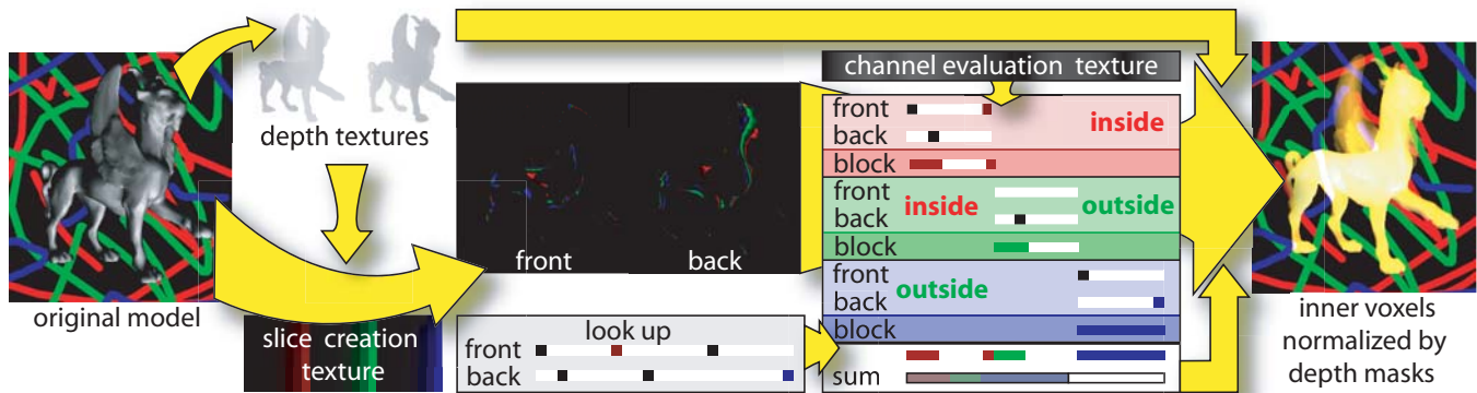
Figure 12: Overview of the refraction algorithm (cp. color plate B1)
