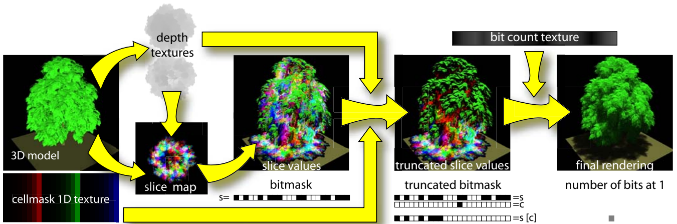
Figure 5: Overview of the transmittance shadow map algorithm - here with 24 slices stored in RGB channels of 8 bits (cp. color plate AI)
