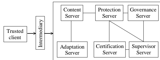
Fig. 1. DMAG-MIPAMS architecture
