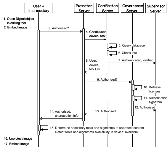
Fig. 2. Content composition use case
