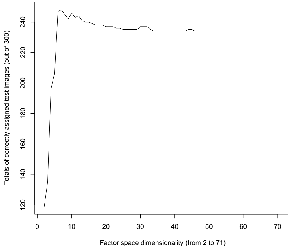
Fig. 10. Totalled correct assignments for best fit Euclidean (factor) subspaces, in dimensions 2 to 71.
