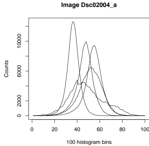
Fig. 2. Distributions of wavelet scales of the image shown in Figure 1. The higher peaked curves are from wavelet scales 1, 3, and 2, respectively, from left to right. The second lowest peaked curve, and the lowest one, are from wavelet scales 4 and 5, respectively.
