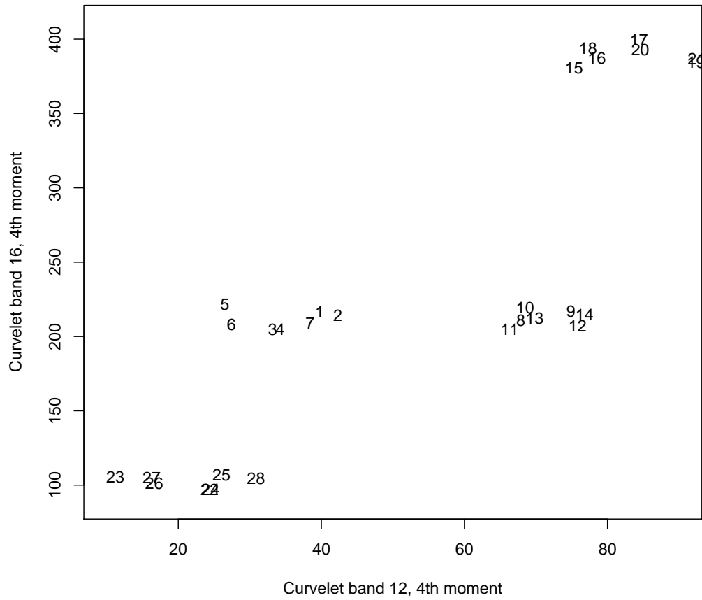
Fig. 7. Identical to Figure 6 but with extensive jitter applied to image labels to avoid the superimposed display.
