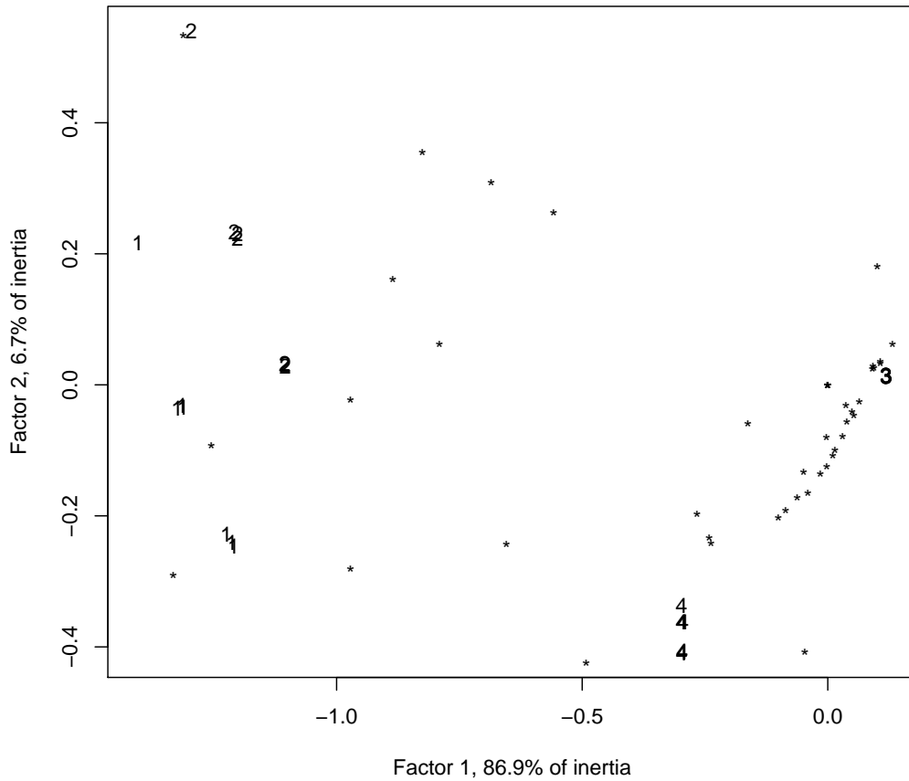
Fig. 4. Principal factor plane. Clusters of images are displayed with 1 for first cluster images, 2 for second, and so on. Features are displayed with an asterisk.
