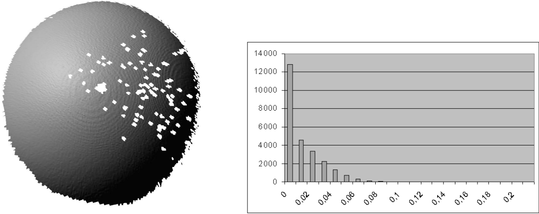
Figure 2. Rendering of a data set acquired with our stripe projection sensor. The object is a precise sphere. Deviations of the sensed data from the ideal sphere are shown on the right. The number of points is plotted over the deviations in millimeters.
