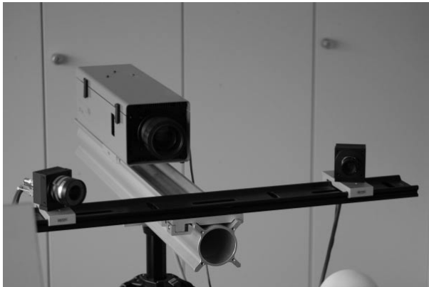
Figure 1. The sensor hardware used for the experiments consists of a LCD stripe projector and a digital camera.
