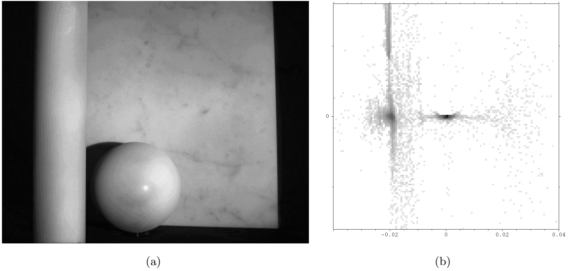
Figure 3. (a) Test scene containing basic shapes as acquired with our stripe projection sensor. (b) Two-dimensional curvature histogram of Gaussian curvature over mean curvature.
