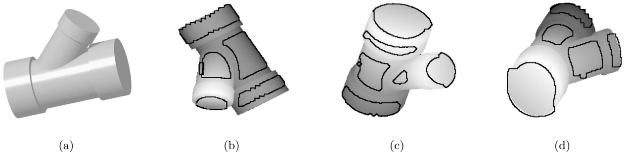
Figure 4. (a) The CAD model of “bigwye”. (b)-(d) Extraction results on test dataset. Classification of surfaces is independent of the pose of the object.
