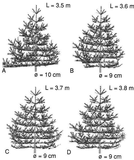
Fig. 4. The effect of the number of sectors in the sky on the appearance of tree simulated with LIGNUM (A, 2 \times 2 , B, 4 \times 4 ; C, 6 \times 6 and D, 10 \times 10 sectors). Also the length of the tree ( L ) and the diameter at base ( \phi ) are presented.
