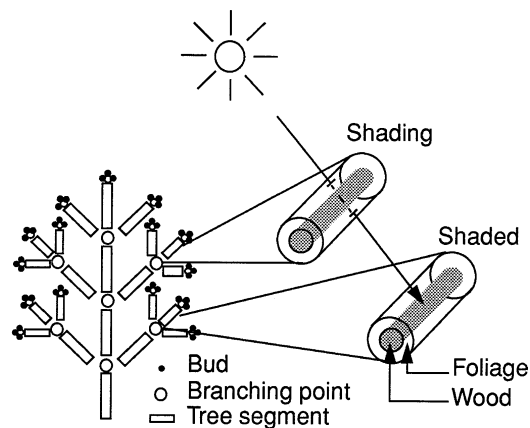
Fig. 1. Schematic presentation of a tree consisting of simple structural units in LIGNUM and the principle of the solar radiation interception model. The distance light beam traverses in foliage is marked by a dashed line.
