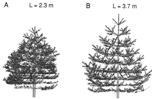
Fig. 6. The effect of branching habit (A, q = 0 , branch order does not affect the length of laterals; B: q = 0.2 , it affects) on outlook and height of the tree ( L ) at the age of 10 years. Diameter at base is in both cases 8 cm.
