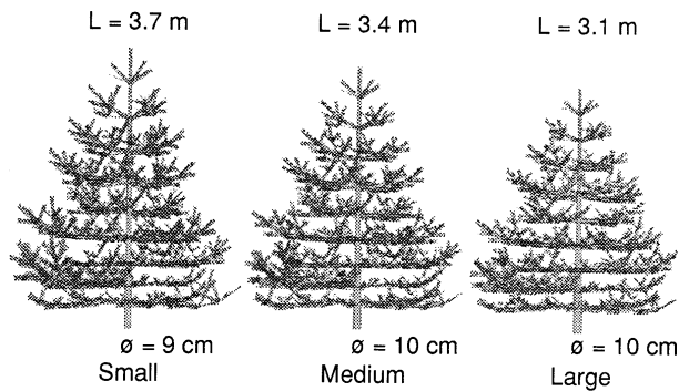
Fig. 5. Simulation of the effect of the rate of sapwood senescence ( S_s = 0.2 , small; S_s = 0.6 , medium; S_s = 1.0 , large) on growth for a 10 year old tree. The length of the tree ( L ) and the diameter at base ( \phi ) are also presented.
