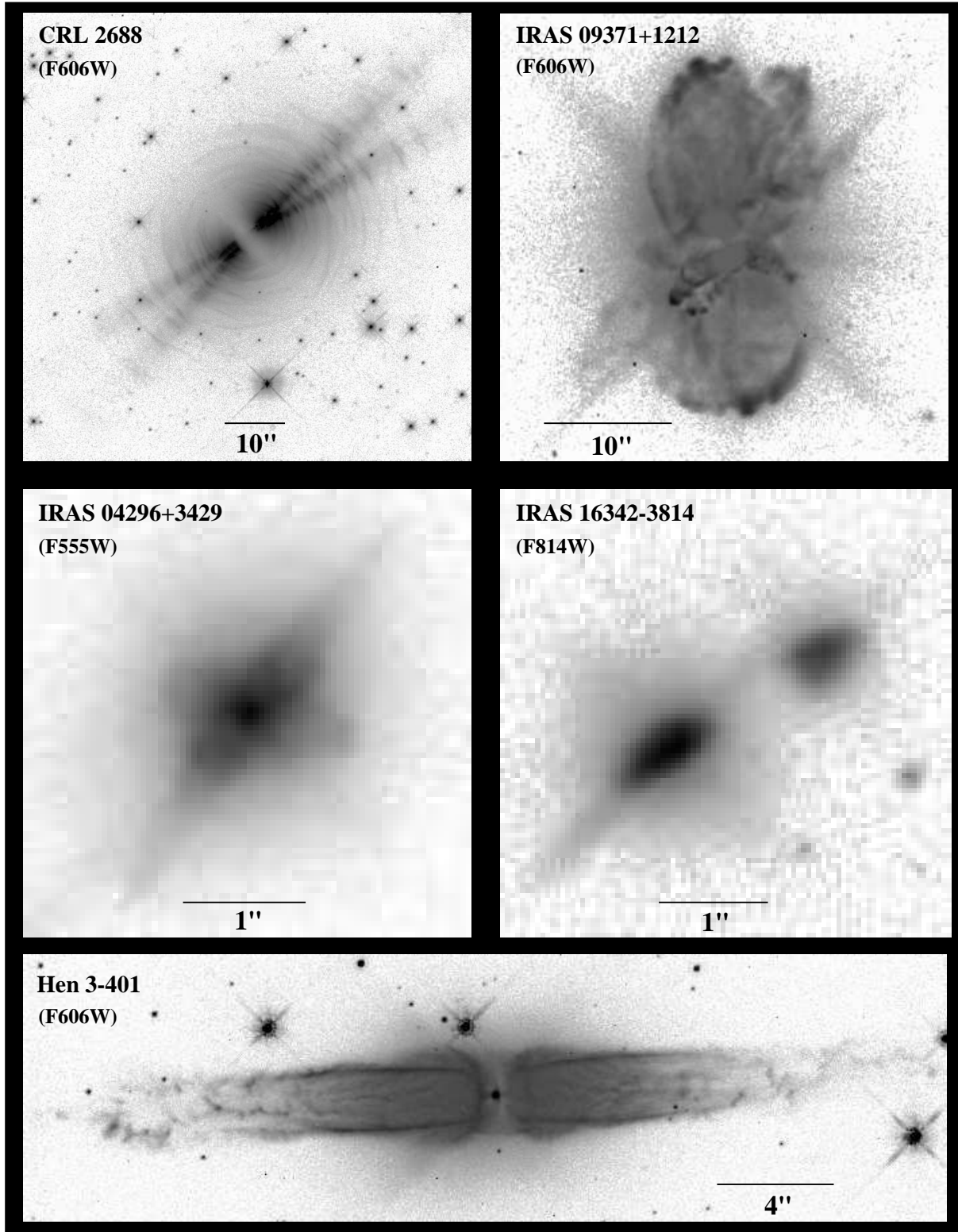
Fig. 1. HST /WFPC2 images (in reverse grey-scale) of selected proto-planetary nebulae. Sharp features have been modestly emphasized in IRAS 09371+1212 (Frosty Leo Nebula) and Hen 3-401 as described in ST98). Note the wide variety of morphologies; the concentric arcs and “searchlight beams” in CRL 2688 (details in Sahai et al. 1998a) and the collimated jet-like lobes near the nebular waist in IRAS 09371+1212 (details in Sahai et al. 2000).
