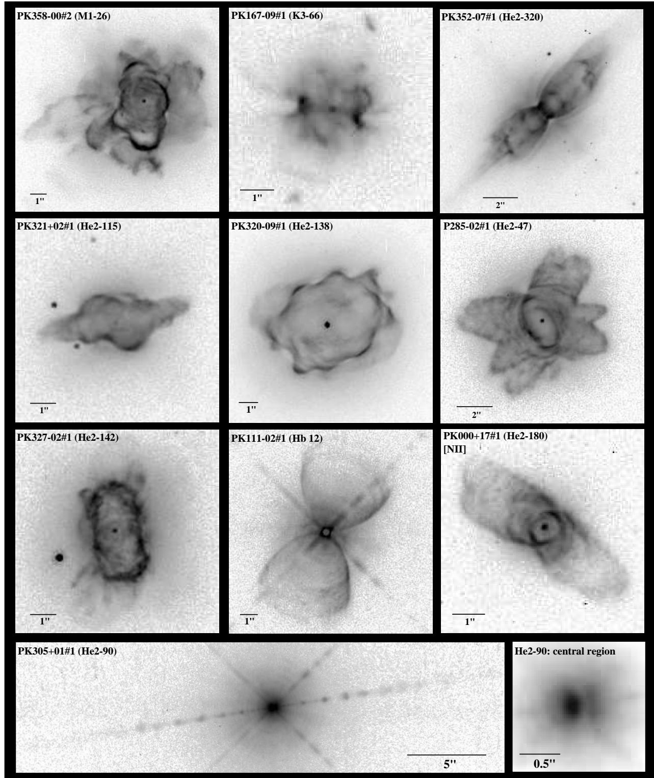
Fig. 2. HST /WFPC2 H\alpha images (in reverse grey-scale) of young planetary nebulae from our survey. Note (a) the wide variety of morphologies, including the plethora of lobes in He2-47 (details in Sahai 2000b), and (b) the amazing morphological similarity of the highly-collimated, pulsed, bipolar jet and central bipolar nebula with obscuring edge-on disk seen in Hen 2-90 to the features seen in low-mass YSOs like HH30 (details in Sahai & Nyman 2000). Sharp features have been emphasized as described in ST98 (the spikes at \pm 45^\circ in the HB 12 & He2-90 images are telescope artifacts).
