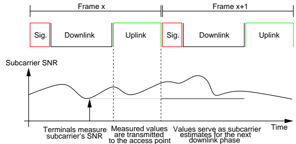
Fig. 4. Process of acquiring subcarrier gain knowledge
