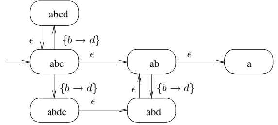
Figure 1. Possible FSM for orderings
