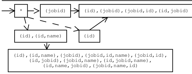
Figure 12. DFSM for NFSM in Figure 11
