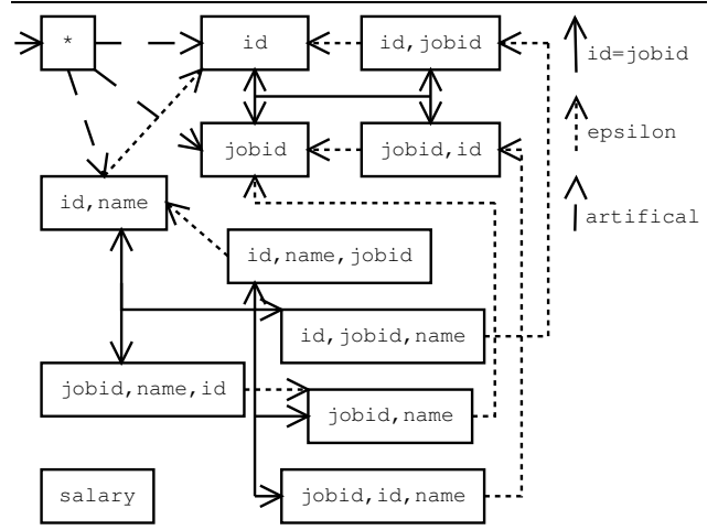
Figure 11. NFSM for a simple query
