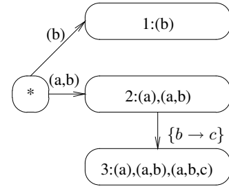
Figure 8. Resulting DFSM
