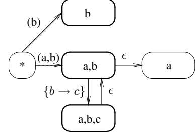
Figure 7. Final NFSM
