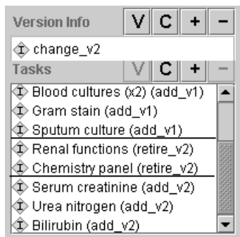
Figure 3. Details of the action step “Laboratory tests”, shown in Figure 2. Instead of using colors to distinguish version information of each slot value, information is represented textually. v1-version 1; v2-version 2.
