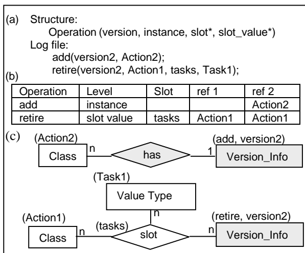
Figure 1. Three ways of representing changes: (a) log file; (b) difference table; (c) version annotations used to extend the CIG ontology. * = optional; ref1, ref2 = references to instance in version 1 and 2. Rectangles denote ontology classes; Diamonds denote relations. Extensions to the CIGs ontology are shown in gray. Instances are shown in parentheses.
