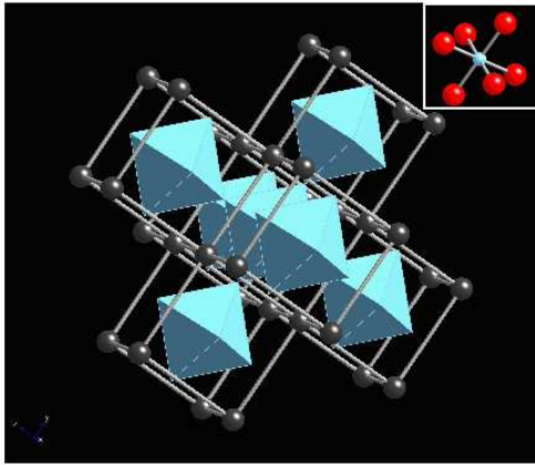
Figure 13: Rendering of the ideal rhombohedral structure of \text{BaTiO}_3 . The structure is a repetition of nearly perfect Ti-O octahedra that are separated by a nearly cubic cage of Ba atoms. The nearly perfect inversion symmetry of the Ti-O octahedra leads to only a small low-energy resonance in the XANES. Except for a mixture of both Ba and Sr atoms on the same site, this is the expected structure for BST films deposited with substrate temperatures.
