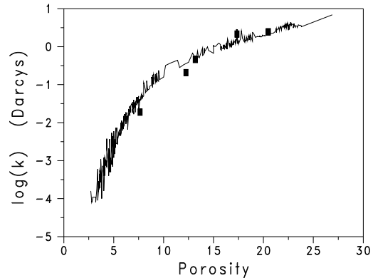
Figure 6: Measured and modeled permeabilities of Fontainebleau sandstone media. The solid rectangles show the modeled results.
