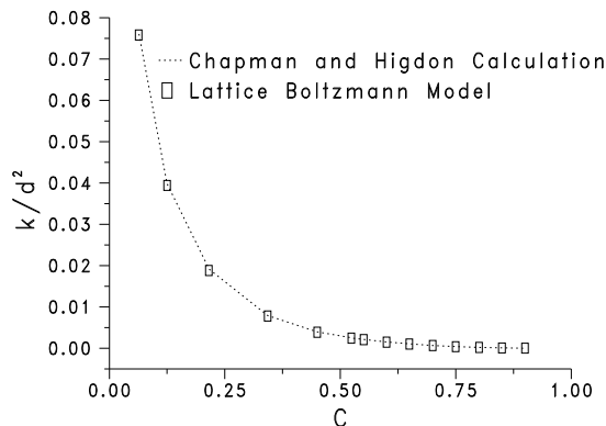
Figure 4: Flow through spheres centered on a simple cubic lattice. The permeability, k , is normalized by the square of the distance, d , between sphere centers.
