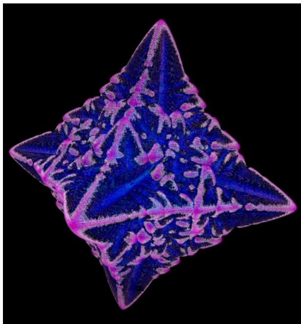
Figure 19: A 3D dendrite visualized using glyphs and semi-transparent colors. This image was generated from the same data as in Figure 17. In this image the output from the simulator has been mirrored along all three axes giving a symmetric six-pointed star structure. The image in Figure 17, due to memory limitations in computing the isosurface, was mirrored only along the x and y axes.
