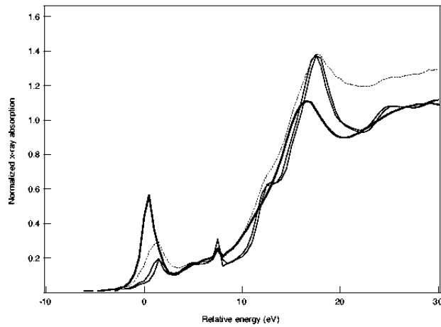
Figure 11: Measured XANES data of 4 Barium-strontium titanate (BST) films deposited by MOCVD. The variation in size and energy position of the pre-edge peak near -2 to +2 eV is a signature of the structural variation in these films.
