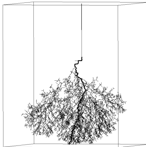
Figure 16: The conical top envelope of the streamer is narrowed by increasing the cutoff-voltage parameter. The narrowing has a counterpart in experimental behavior under increased pressure.
