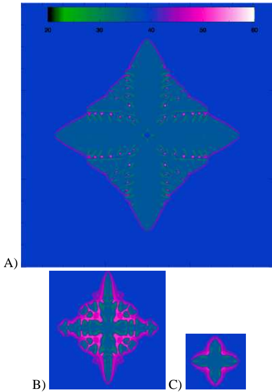
Figure 18: Three 2D slices through the 3D dendrite shown in Figure 17. The scale is the same in these three images but in order to save space the area surrounding the dendrite has been clipped. The color coding used in these images is identical to the color coding used in Figure 17. The blue background corresponds to the initial concentration of approximately 40%. Image A is a slice through the base of the dendrite, image B is a slice 1/4 of the distance from the base of the dendrite to the edge of the volume, and image C is a slice 1/2 of the distance of the way from the center to the edge of the volume.
