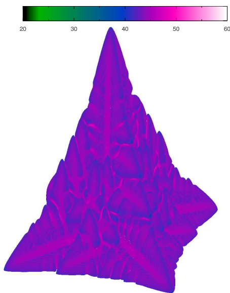
Figure 17: A 3D dendrite from a simulation over a grid of 300^3 points. The color bar shows the coding of the relative concentration of the metals in the dendrite. The color coding ranges from 20%(80%) to 60%(40%).
