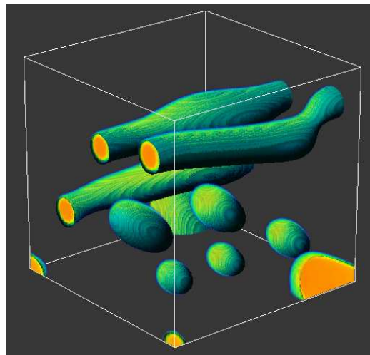
Figure 3: Phase separating binary mixture under shear simulated using a lattice Boltzmann method.
