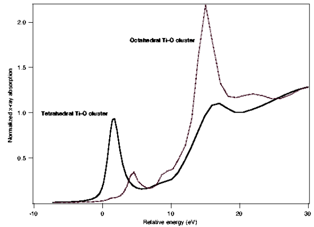
Figure 12: XANES calculation from the octahedral and tetrahedral Ti-O structures shown in Figure 13 and 14. The nearly perfect inversion symmetry of the Ti-O octahedra leads to only a small low-energy resonance in the XANES. The non-inversion symmetric tetrahedral Ti-O environment gives a much larger low-energy resonance. The qualitative similarity of these simulations with the XANES measurements shown in Figure 11 indicates that the BST films make a transition from a non-ferroelectric phase with tetrahedral Ti-O oxygen coordination to the octahedral Ti-O structure that is characteristic of \text{BaTiO}_3 .
