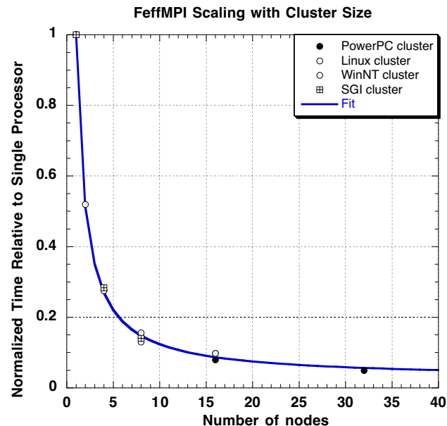
Figure 10: Runtime of a typical FeffMPI XANES calculation with cluster size. The calculation has been run on 4 different clusters. The execution time on a single processor has been normalized to 1.0, showing that the scaling on all clusters is very similar, once the variation in processor speed and compiler quality is eliminated. The scaling indicates that about 3% of the runtime is still from the sequentially executing parts of the code, implying that a very large cluster should run FeffMPI about 30 times faster than an equivalent single processor.
