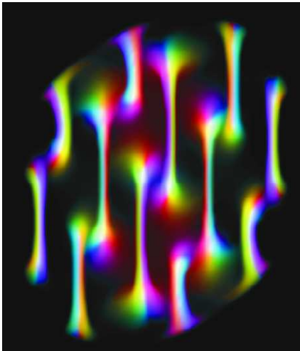
Figure 1: Array of vortices in a Bose-Einstein condensate under rotation.
