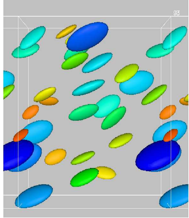
Figure 8: Motion of twenty eight ellipsoidal inclusions, of size varying up to a factor of two, subject to shear. Note that the Jefferies orbits are suppressed due to hydrodynamic interactions between ellipsoids.
