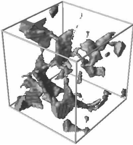
Figure 5: 64^3 portion of the 7.5 % porosity Fontainebleau sandstone media. The solid matrix is made transparent to reveal the pore space (grey shaded region).
