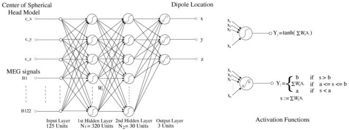
Figure 13. Training datasets were loaded into this MLP structure. Note that the input includes the coordinates of the center of a sphere fit to the subject’s head.
