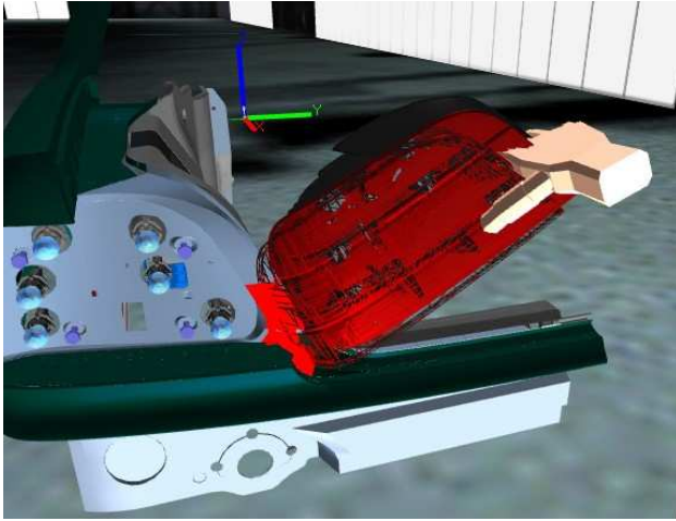
Figure 6: All the algorithms and paradigms presented in this paper have been integrated in our VR system Virtual Design II , which is used by car industries to carry out virtual assembly simulation in scenarios like the two shown above.
