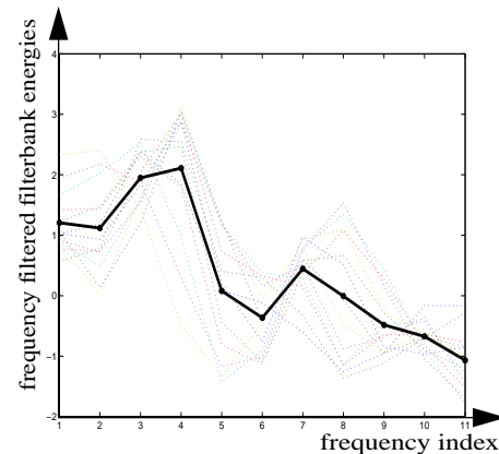
Figure 3: Energy spectrum of a pronunciation of phoneme 'ay'. Each line in the figure corresponds to one time step, and thus to one feature vector (the thick black line is the mean).
