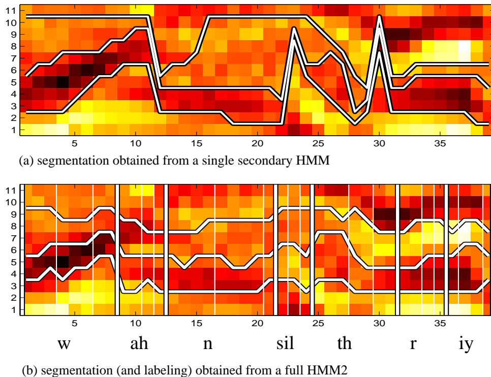
Figure 8: Segmentations obtained (on unseen data) from (a) a single secondary HMM and (b) a full HMM2 system. In both figures, the horizontal lines correspond to the frequency segmentation. In (b), the vertical lines show the temporal segmentation obtained from the full HMM2 system, where phoneme boundaries are displayed as thick lines, and transitions between temporal states of the same phonemes as thin ones.
