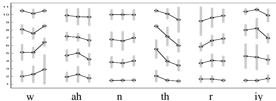
Figure 5: Trained HMM2 parameters for different phonemes. In each column, the means of the frequency indices of the 4 secondary HMM states belonging to the same temporal state are visualized. Vertical bars show the respective variances. The 3 columns belonging to a phoneme correspond to the 3 temporal states.
