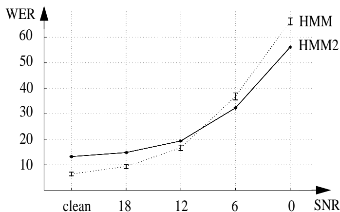
Figure 7: HMM vs. HMM2 performance for frequency filtered filterbank features, illustrated by the dotted and solid lines respectively. Errorbars for HMM WER show the 95% confidence intervals. The results are for clean speech and car noise at different SNR.
