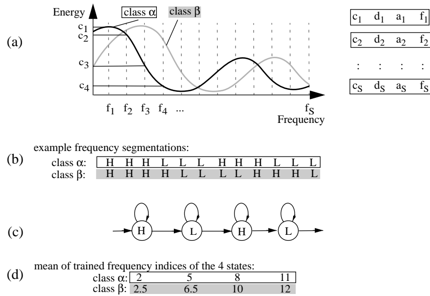
Figure 4: The frequency index: In (a), data assumed to be typical of the classes \alpha and \beta are visualized by a black and a gray curve respectively. On the right, feature vectors (corresponding to the class \alpha curve) as used in the secondary HMM composed of coefficients c_s , their delta d_s , and acceleration coefficients a_s , as well as the frequency coefficient f_s , are shown. In (b), an example frequency segmentation is shown for each class. (c) shows a structure of an HMM with alternating H and L states, which is able to model both classes. With an additional trained frequency coefficient (as shown in (d)), discriminability can be ensured.
