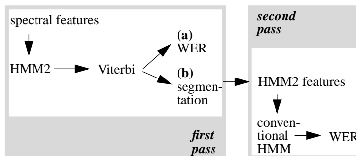
Figure 6: HMM2 system used directly for speech recognition (a), and for features extraction (b). For (b), a second recognition pass, using a conventional HMM, is performed.
