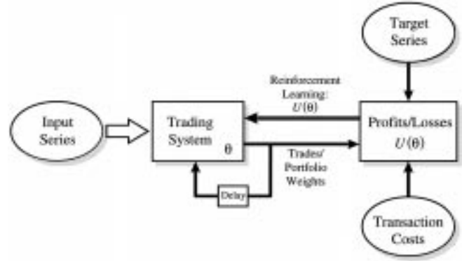
Fig. 1. A trading system based on DR, the approach taken in this paper. The system trades the target series, making trading decisions based upon a set of input variables and the current positions held. No intermediate steps such as making forecasts or labeling desired trades are required and it is not necessary to learn a value function. The trader learns a strategy via trial and error exploration, taking actions and receiving positive or negative reinforcement based on the results. A trading performance function U(\theta) such as profit, utility or risk-adjusted return is, hence, used to directly optimize the trading system parameters \theta . The system is recurrent; the feedback of system state (current positions or portfolio weights) enables the trading system to learn to correctly incorporate transactions costs into its trading decisions. For the traders considered in this paper, the DR (policy search) method of recurrent reinforcement learning is used to optimize the trader.
