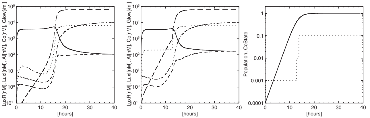
Figure 6. Time evolution of concentrations (in nM) during population growth: proteins LuxR (solid), LuxI (dotted), Ai (dot-dashed), Co (dashed), and total luminescence (long dashes): (a) continuous model, (b) switched model. (c) Population growth curve. The switch history for the hybrid model is dotted.
