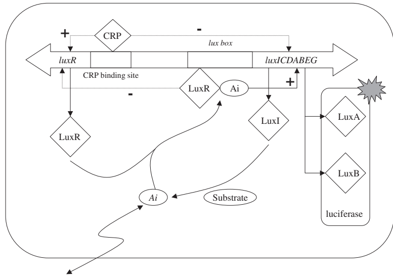
Figure 5. A portion of DNA showing the luxR (transcribed from the leftward operon O_L ) and luxICDABEG (transcribed from the rightward operon O_R ) genes and the binding sites for complex Co and CRP.
