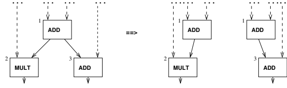
Figure 2: Transforming SSA DAGs into SSA Trees
