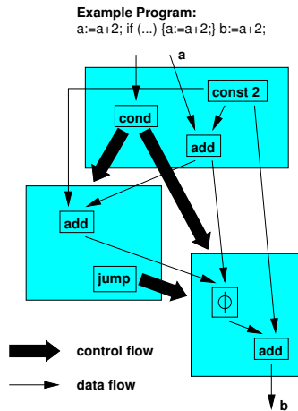
Figure 1: SSA Representation
