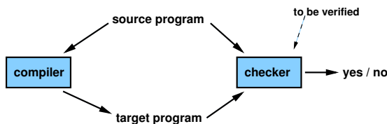
Figure 3: Program Checking
