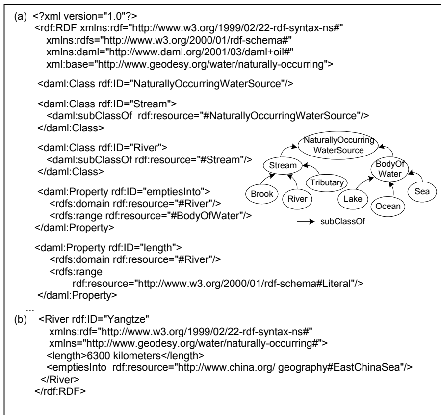
Fig. 1. NaturallyOccurringWaterSource in DAML+OIL (a) Ontology (b) Resource instance
