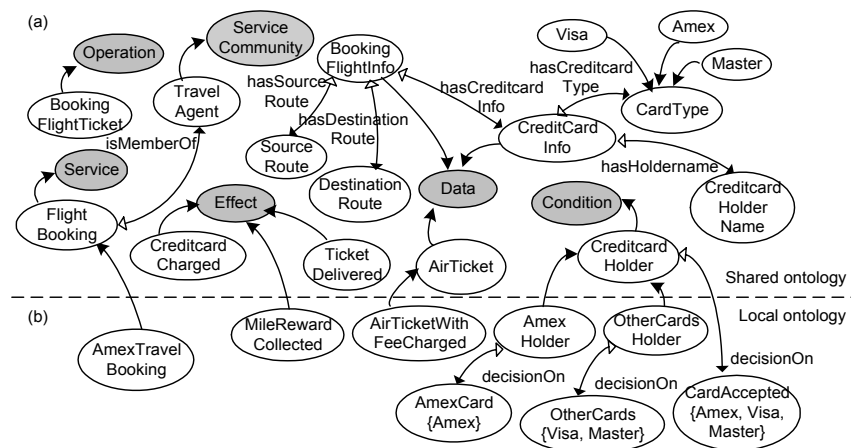
Fig. 3. Service ontology
