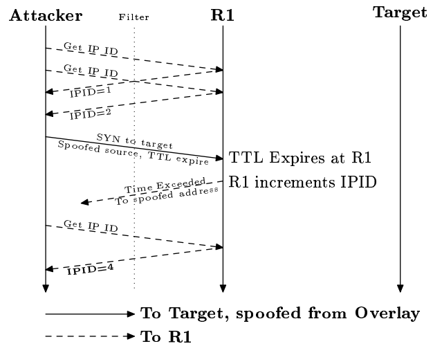
Figure 6: Next-hop scan. This attack combines the idlescan and firewalking to determine from an interior router if packets get through the firewall.
