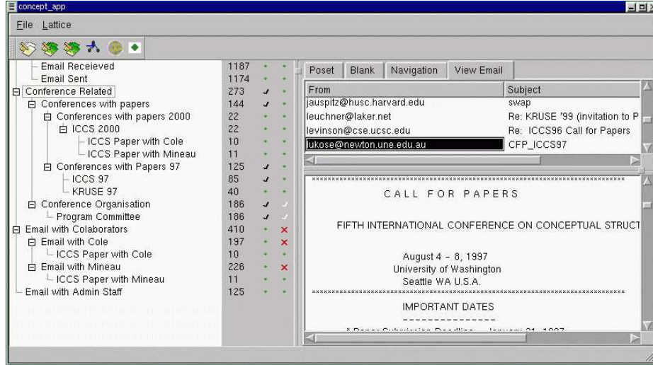
Fig. 4. Interface for viewing email and associating email with catchwords
