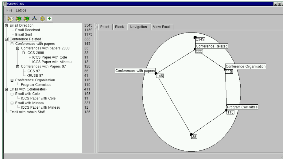
Fig. 5. Concept Lattice derived from the Scale for “Conference Related”.
