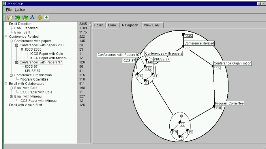
Fig. 6. Concept Lattice derived from the Scales for “Conference Related” and “Conferences with Papers”.
