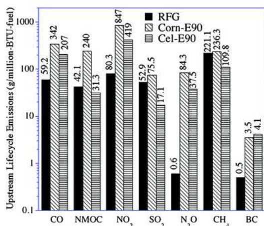
Fig. 3 Upstream lifecycle emissions of several individual pollutants from corn-E90 and cellulosic-E90 relative to reformulated gasoline (RFG). 58
