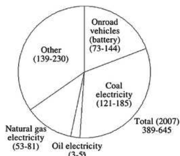
Fig. 9 Thousands of 5 MW wind turbines needed, placed in locations where the mean annual wind speed is 7.0 \text{ m s}^{-1} (high number) to 8.5 \text{ m s}^{-1} (low number), to displace 100% of US \text{CO}_2 from each source. Onroad vehicles include light and heavy-duty vehicles and are assumed to be replaced by BEVs. See ESI† for calculations. The corresponding sources of the 5970 MT- \text{CO}_2 emitted in the US in 2007 are onroad vehicles: 24.6%, coal electricity: 32.8%, oil electricity: 0.91%, natural gas electricity: 6.1%, and other: 35.7%.
