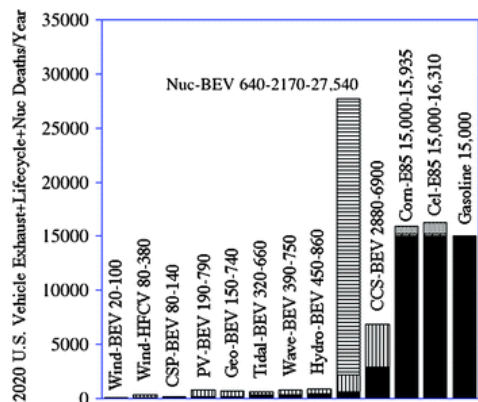
Fig. 4 Estimates of future (c. 2020) US premature deaths per year from vehicles replacing light- and heavy-duty gasoline onroad vehicles and their upstream emissions assuming full penetration of each vehicle type or fuel, as discussed in the text. Low (solid) and high (solid+vertical lines) estimates are given. In the case of nuclear-BEV, the upper limit of the number of deaths, scaled to US population, due to a nuclear exchange caused by the proliferation of nuclear energy facilities worldwide is also given (horizontal lines). In the case of corn-E85 and cellulosic-E85, the dots are the additional US death rate due to upstream emissions from producing and distributing E85 minus those from producing and distributing gasoline (see text) and the slanted lines are the additional tailpipe emissions of E85 over gasoline for the US. 25
